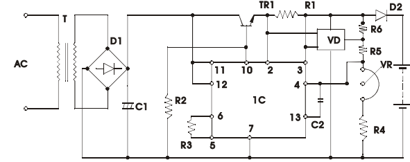
Figure 16. EXAMPLE OF A TWO STEP CONSTANT VOLTAGE CONSTANT-CURRENT CHARGE CIRCUIT
